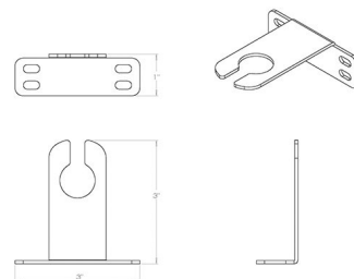
5000-GM-BZ Line Drawing
