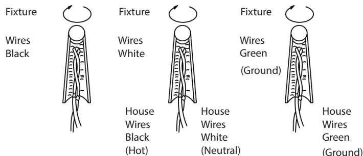
Wiring Diagram Fig.1
