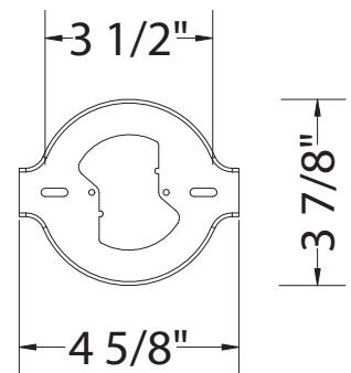
Mounting Back plate Dimensions
