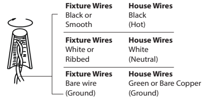
Fig.2 Wiring
