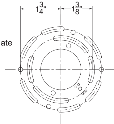
Mounting Hole Dimensions
