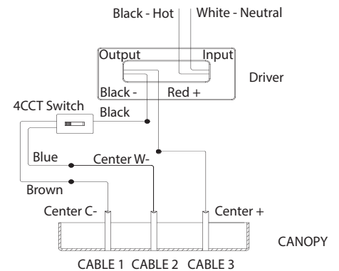
Fig.5 Driver Wires
