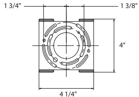
Fig.3 Mounting Plate Dimensions
