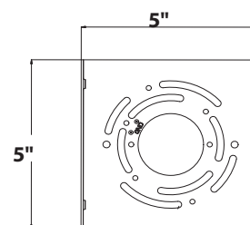
Mounting Plate Dimensions
