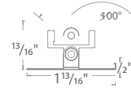
ADJUSTABLE CHANNEL CLIP LED-T-CL2-PT
