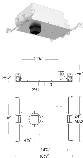
Square, New Construction Millwork
